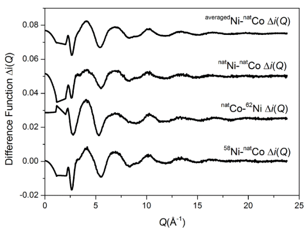
Figure 5. First order difference isomorphous substitution functions \Delta i(Q) .
