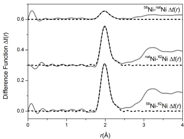
Figure 4. Real space data for the isotopic substitution difference functions. The solid curve represents the experimental data and the broken curve represents the resultant fits.
