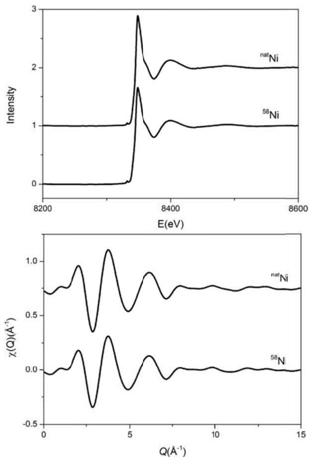
Figure S1. (a) Normalised EXAFS data for ^{58}\text{Ni} and ^{\text{nat}}\text{Ni} , (b) reciprocal space data. Data sets are offset for clarity.
