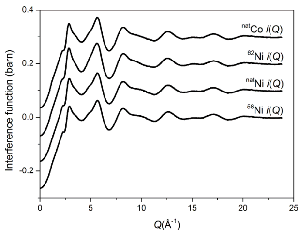
Figure 1. Total interference functions for the Ni and Co doped bioactive glasses.
