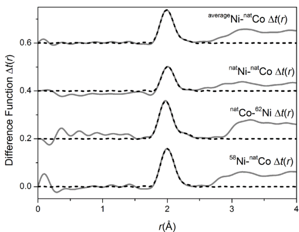
Figure 6. Real space data for the isomorphous substitution difference functions. The solid curve represents the experimental data and the broken curve represents the resultant fits.
