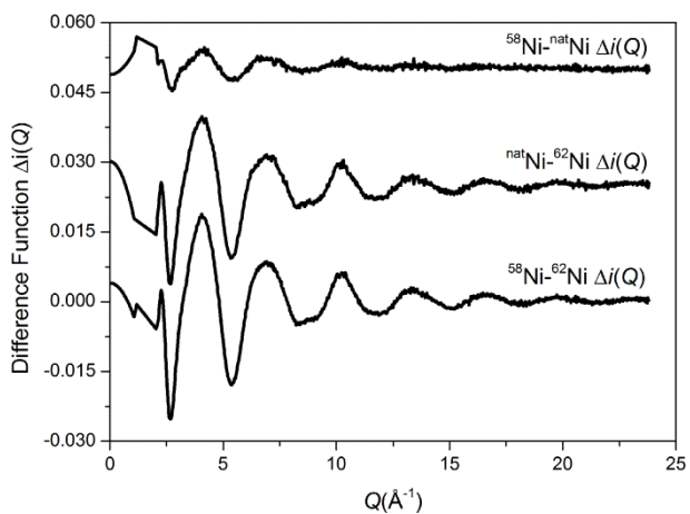
Figure 3. First order difference isotopic substitution functions \Delta i(Q) .
